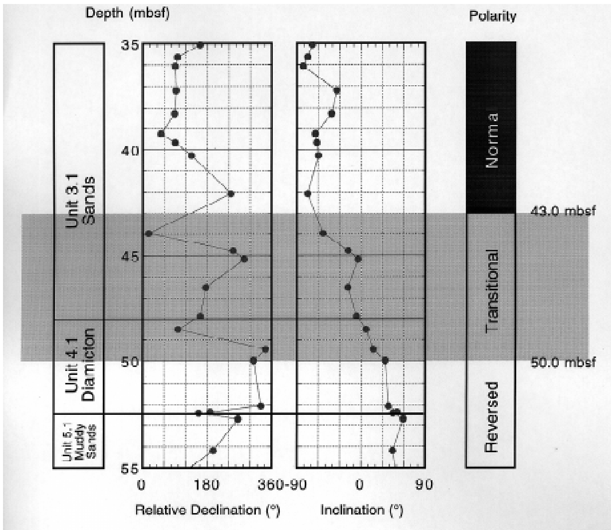
Fig. 7 - Variations in palaeomagnetic declination (arbitrary) and inclination (identified from principal component analysis of multiple demagnetization steps) through the inferred geomagnetic polarity transition (shaded) between magnetozones R2 and N2. The drillcore is not oriented with respect to north. The transition crosses the contact between lithostratigraphic units 4.1 and 3.1 and provides an estimate of accumulation rates and of rates of glacial processes (see discussion in text).
