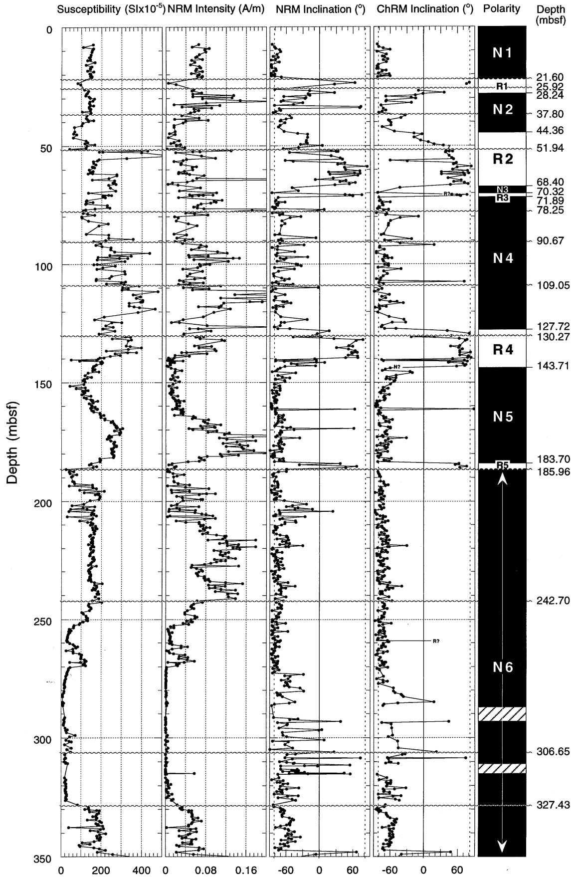
Fig. 2 - Down-core variations of magnetic susceptibility, natural remanent magnetization (NRM) intensity, NRM inclination, inclination of the characteristic remanent magnetization (ChRM) component and the magnetic polarity zonation (black = normal polarity, white = reversed polarity) for the CRP-2/2A drillcore. R? (N?) denotes samples that display a clear trend toward reversed (normal) polarity but for which a stable ChRM was not reached before the remanence intensity became too weak to measure. Hatching represents intervals where it was not possible to determine polarity due to poor drillcore recovery, unsuitable lithologies, intraformational deformation, or where it was not possible to determine ChRM directions.
