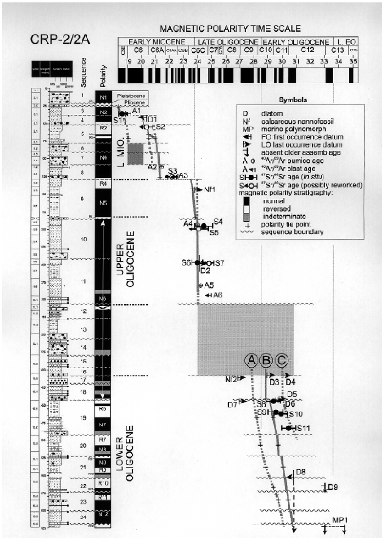
Fig. 10 - Correlation of the CRP-2/2A magnetic polarity zonation with the magnetic polarity time scale (MPTS) of Cande & Kent (1995) and Berggren et al. (1995). Black (white) denotes normal (reversed) polarity. Grey denotes intervals where it was not possible to determine the polarity due to unstable palaeomagnetic behaviour or to sampling gaps. The interval between 311 and 315.52 mbsf is an intraformational breccia and did not yield useful polarity data. Solid lines indicate preferred age-depth correlations; stippled lines indicate other possible correlations (see discussion in text). The shaded area represents the range of possible correlations between 306.65 and 409.36 mbsf where no correlation is possible with existing data. Wilson et al. (this volume) lists datum events, with alpha-numeric indicators. See text for discussion.
